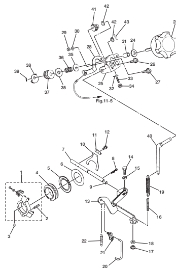
Fig. 8 GOVERNOR ガバナ
