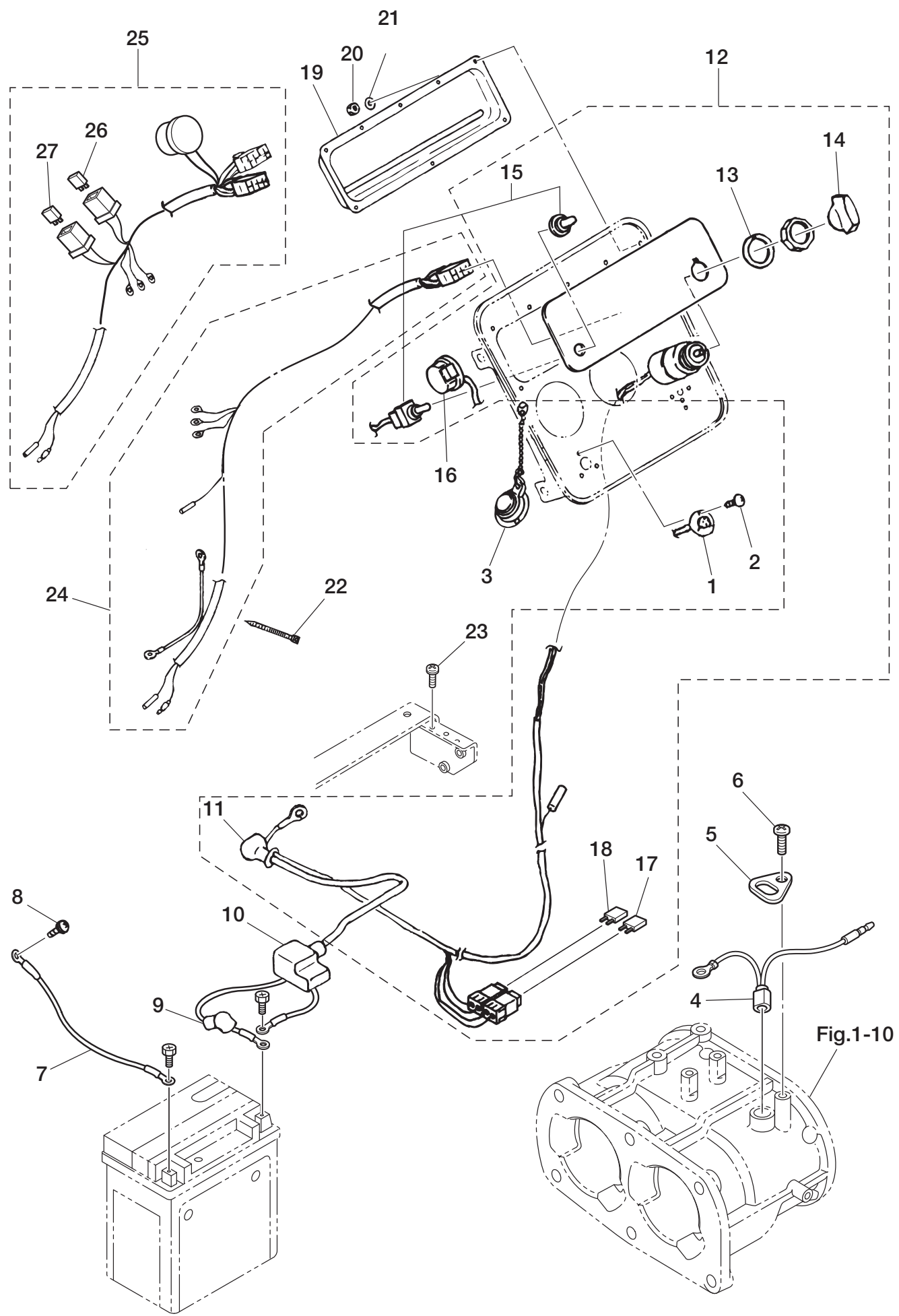
Fig. 10B ELECTRIC PARTS (VC82AS, VC82/85BS)
